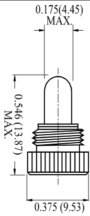
T-1 1/4 Knurled Screw Base
